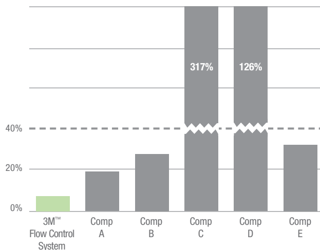
Dispensing System Average % Dilution Error (dispensers tested over a dynamic water pressure range of 20–120 psi)
